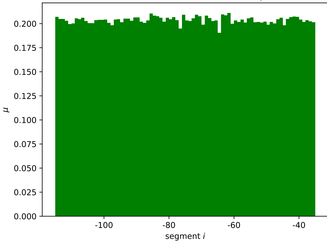
pitA mean wildtype expression \mu_i^*
