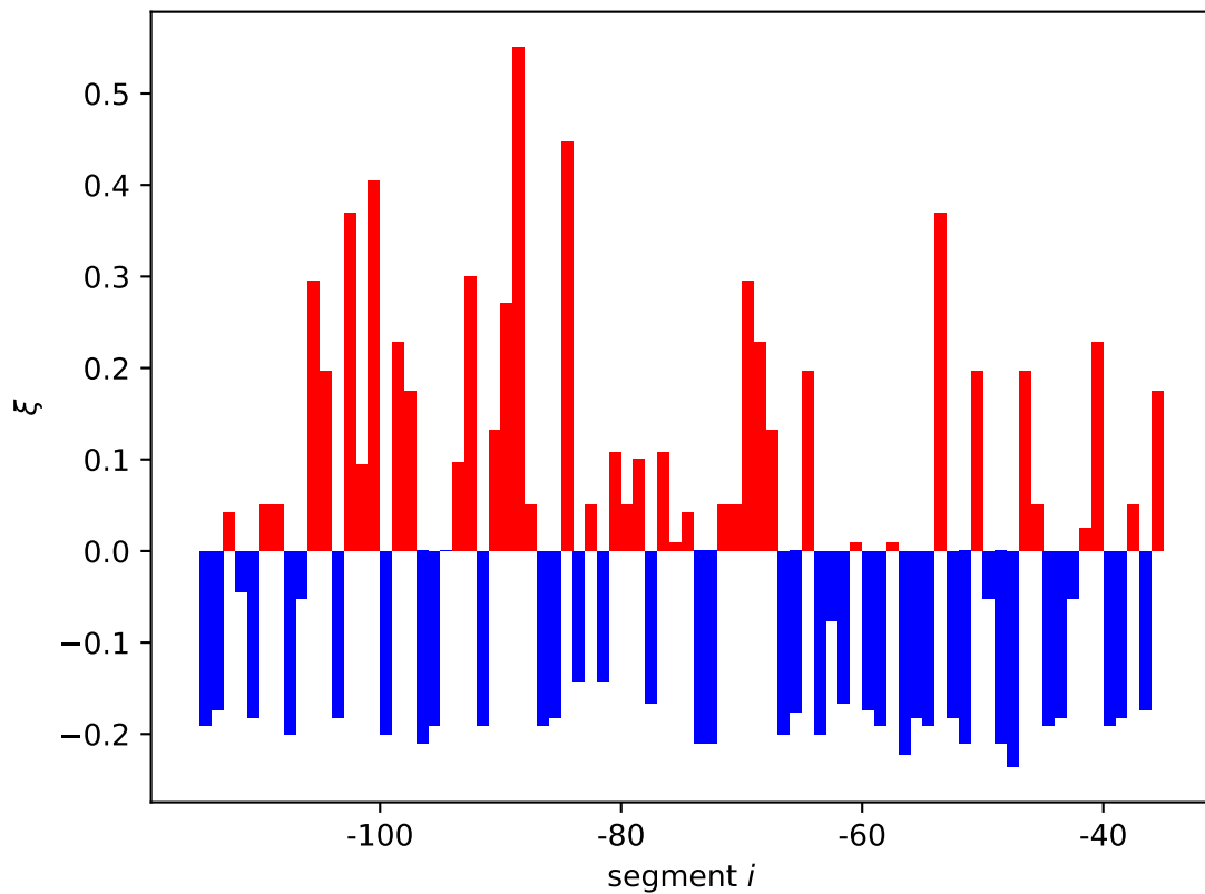
poxB expression shift \xi_i[01, 10]
