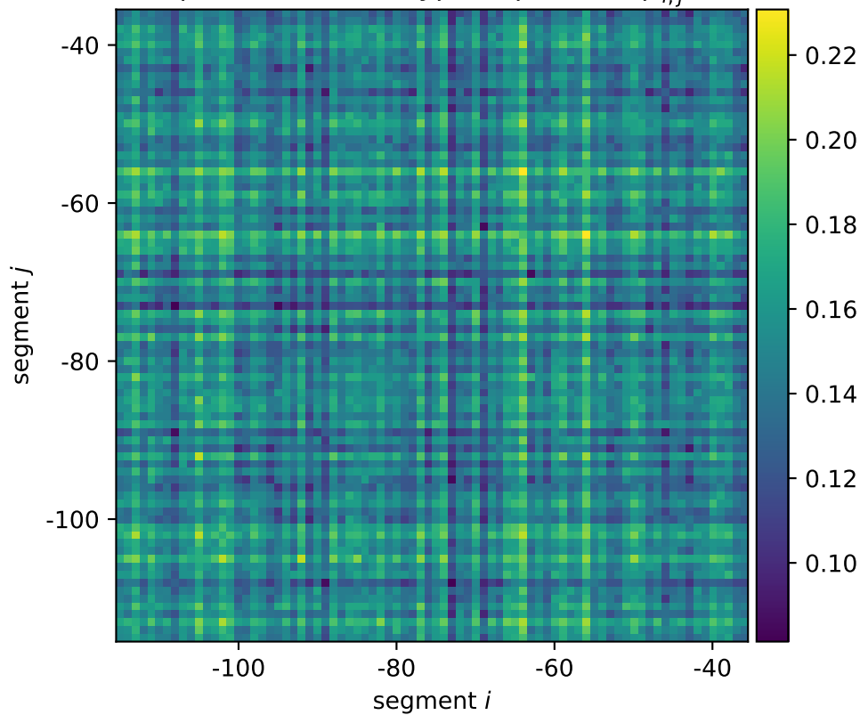
poxB mean wildtype expression \mu_{i,j}^*
