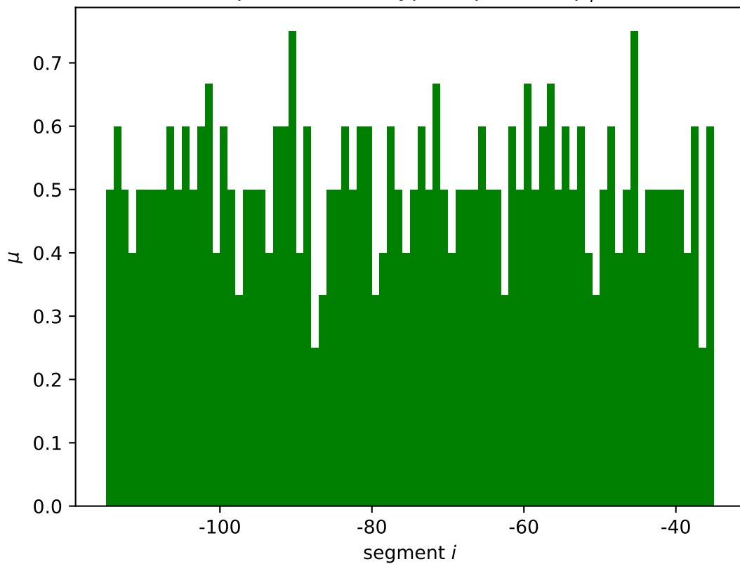
rapA mean wildtype expression \mu_i^*
