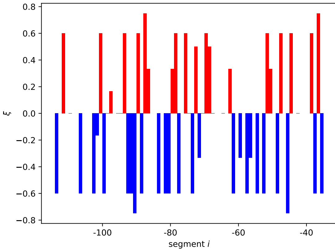
rapA expression shift \xi_i[01, 10]
