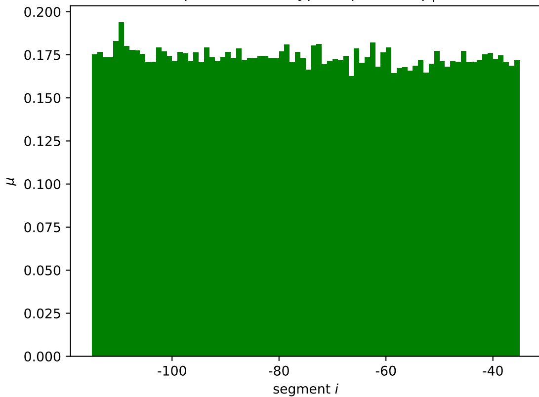
rapA mean wildtype expression \mu_i^*
