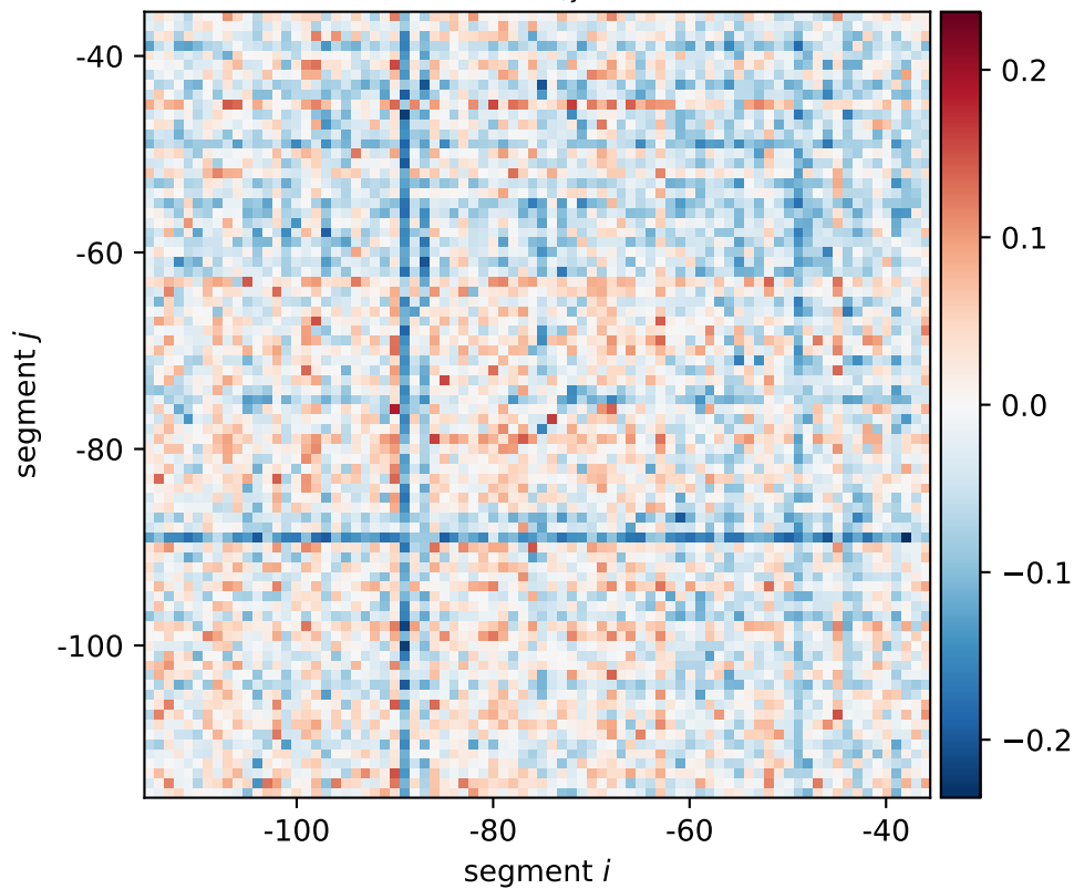
rscF expression shift \xi_{i,j}[0101, 0110, 1010]
