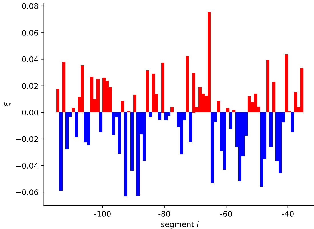
rscF expression shift \xi_i[01, 10]
