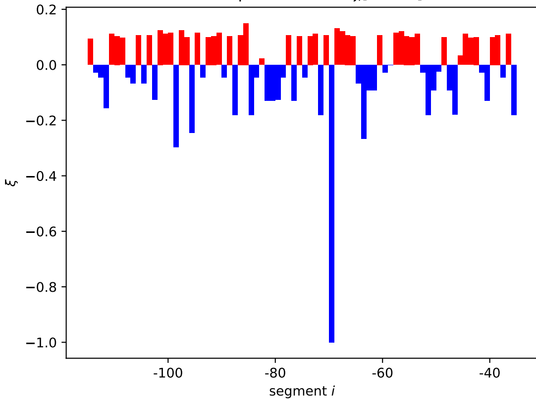
rcsF expression shift \xi_i[01, 10]
