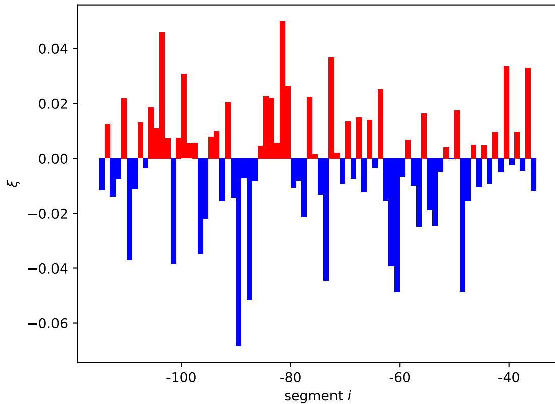
rlmA expression shift \xi_i[01, 10]
