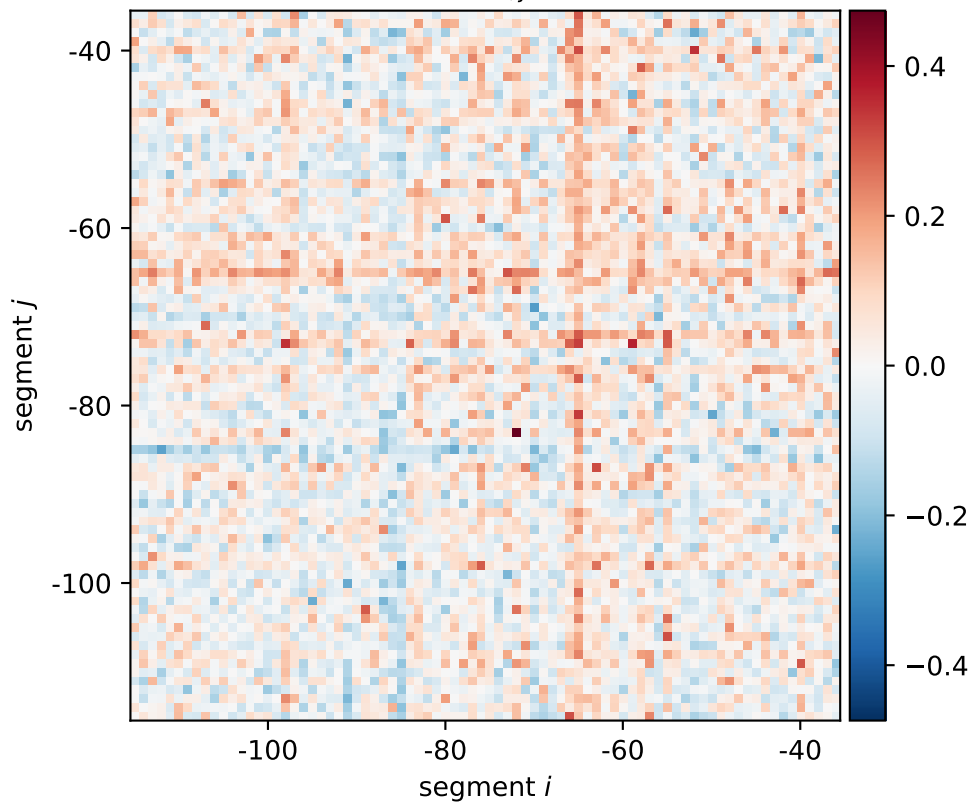
rspA expression shift \xi_{i,j}[0101, 0110, 1010]
