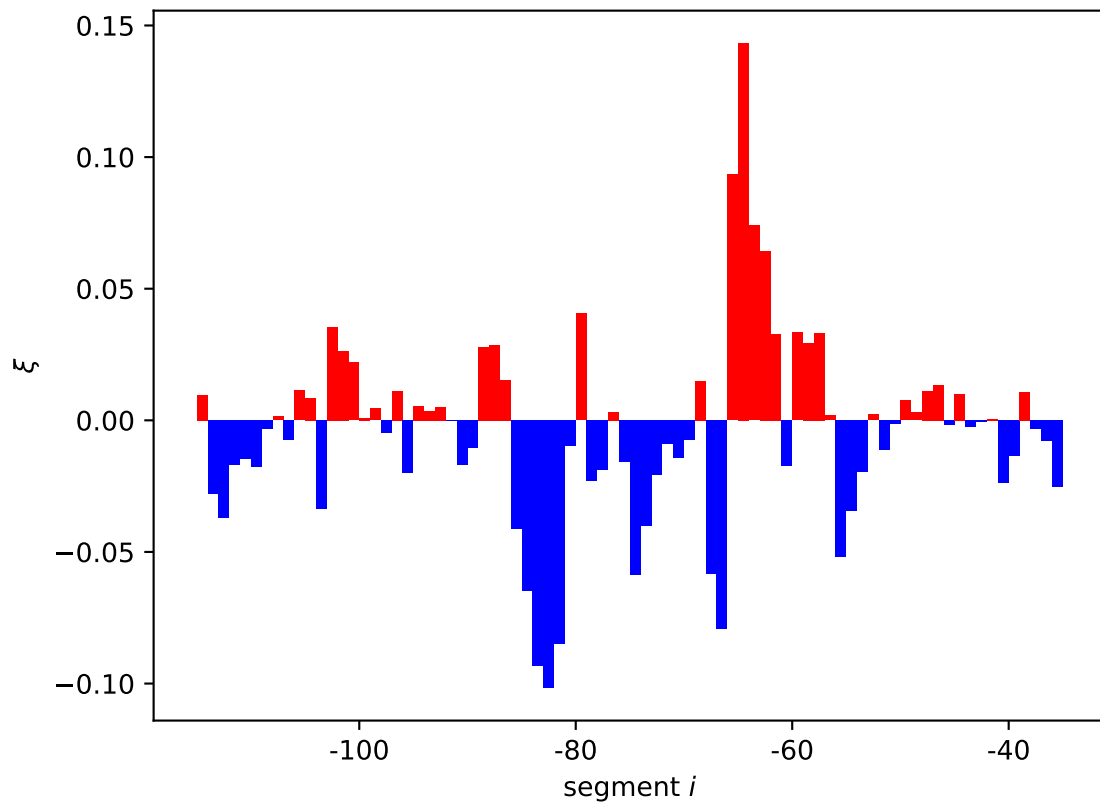
rspA expression shift \xi_i[01, 10]
