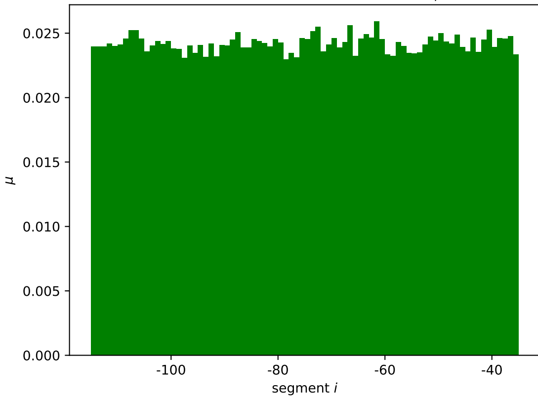
rumB mean wildtype expression \mu_i^*
