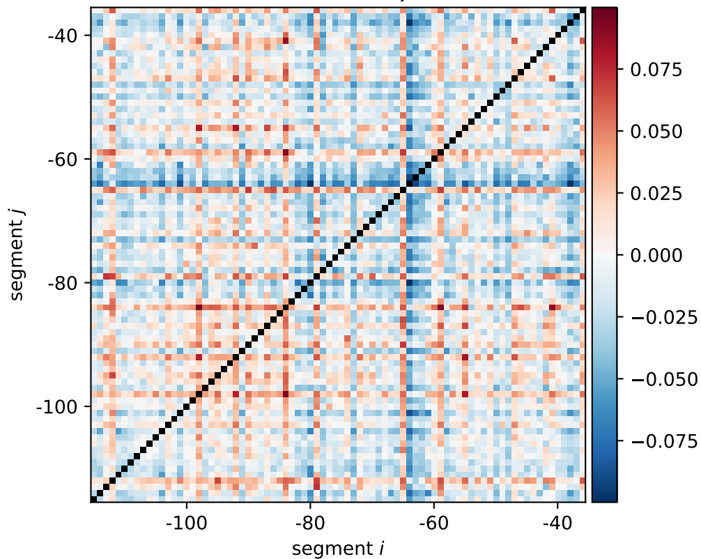
rumB expression shift \xi_{i,j}[0011, 1100]
