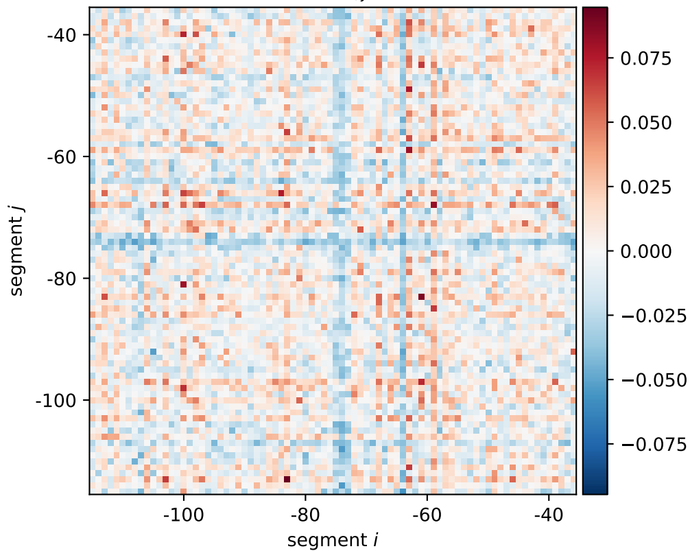
rumB expression shift \xi_{i,j}[0101, 0110, 1010]
