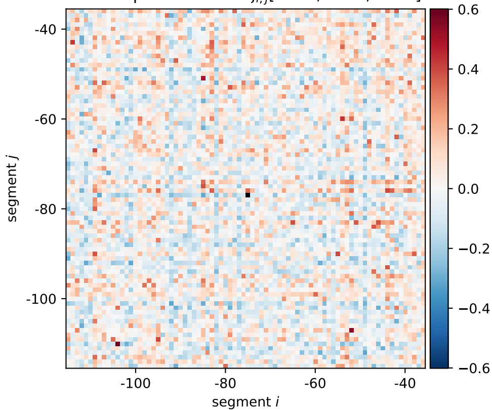
sbcB expression shift \xi_{i,j}[0101, 0110, 1010]
