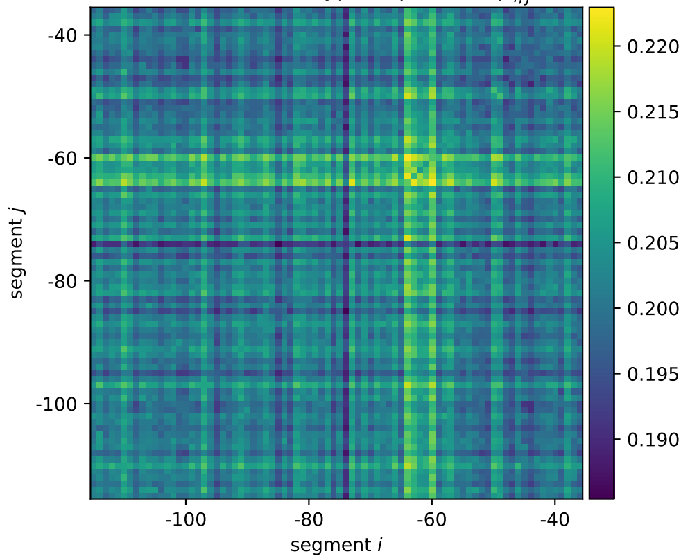
sbcB mean wildtype expression \mu_{i,j}^*
