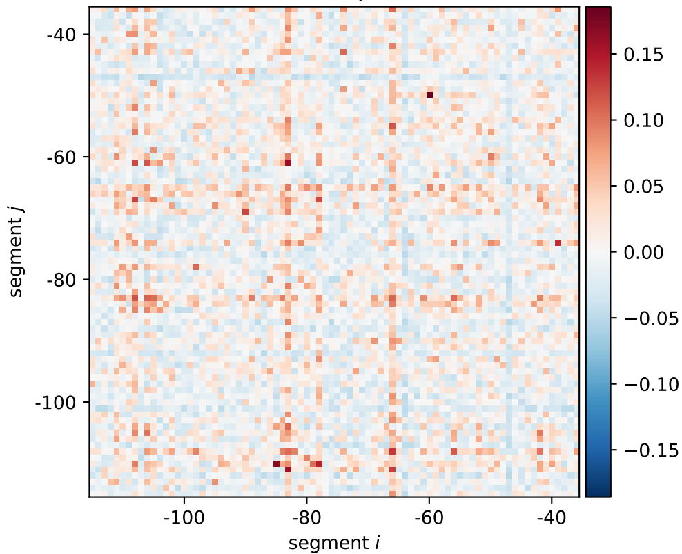
sdaB expression shift \xi_{i,j}[0101, 0110, 1010]
