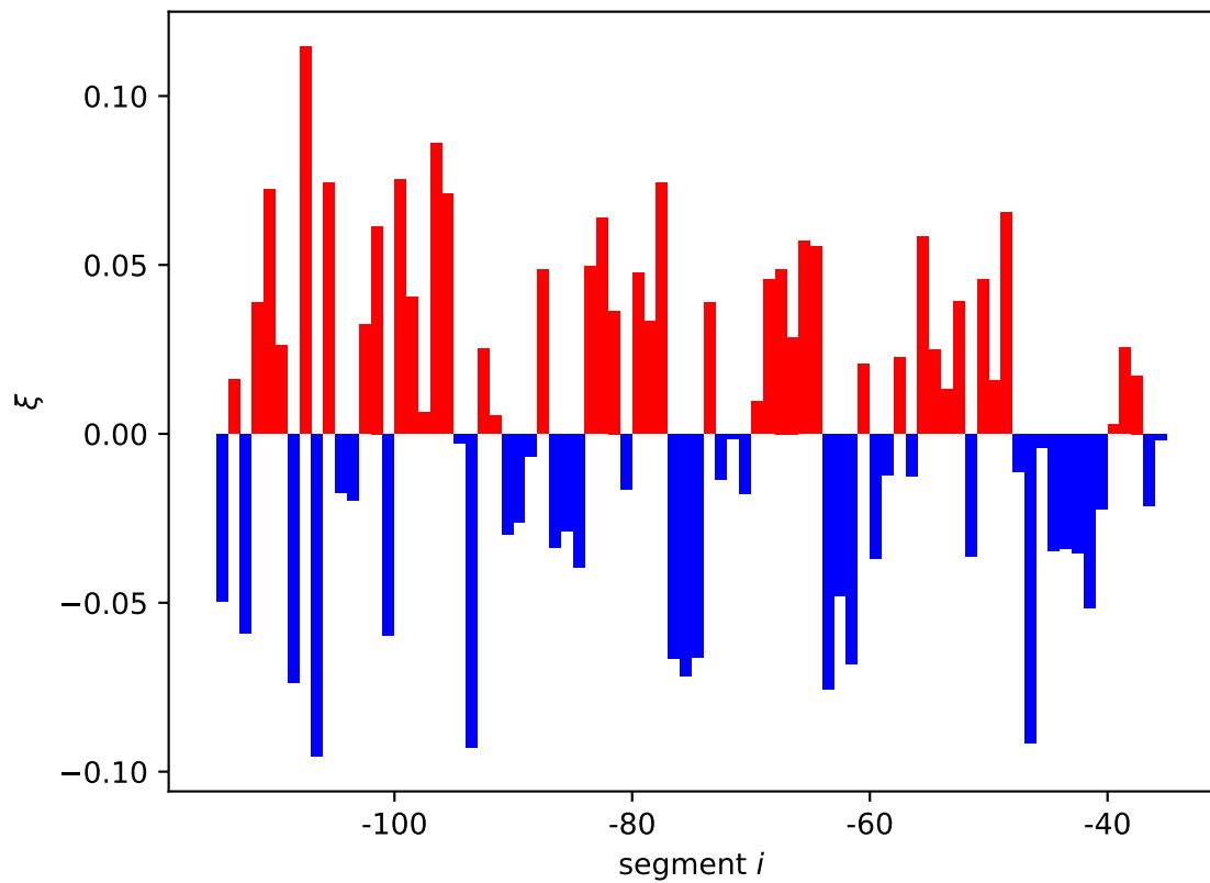
sdaB expression shift \xi_i[01, 10]
