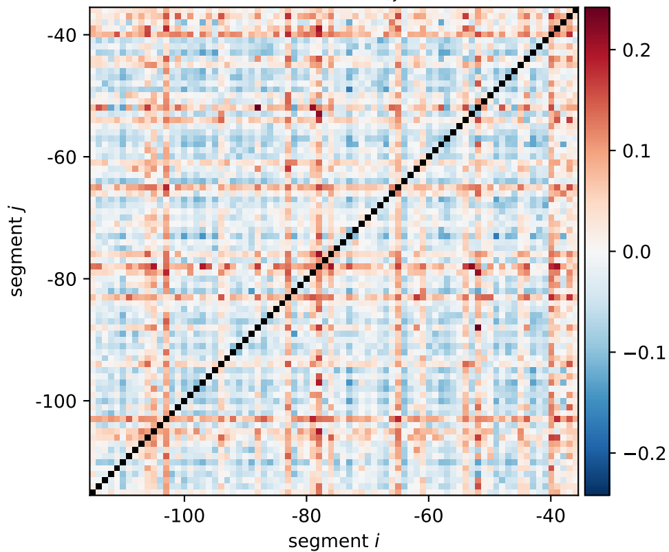
sdaB expression shift \xi_{i,j}[0011, 1100]
