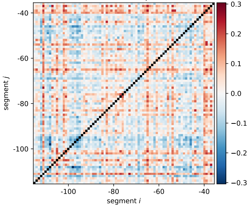
sdaB expression shift \xi_{i,j}[\text{0011}, \text{1100}]
