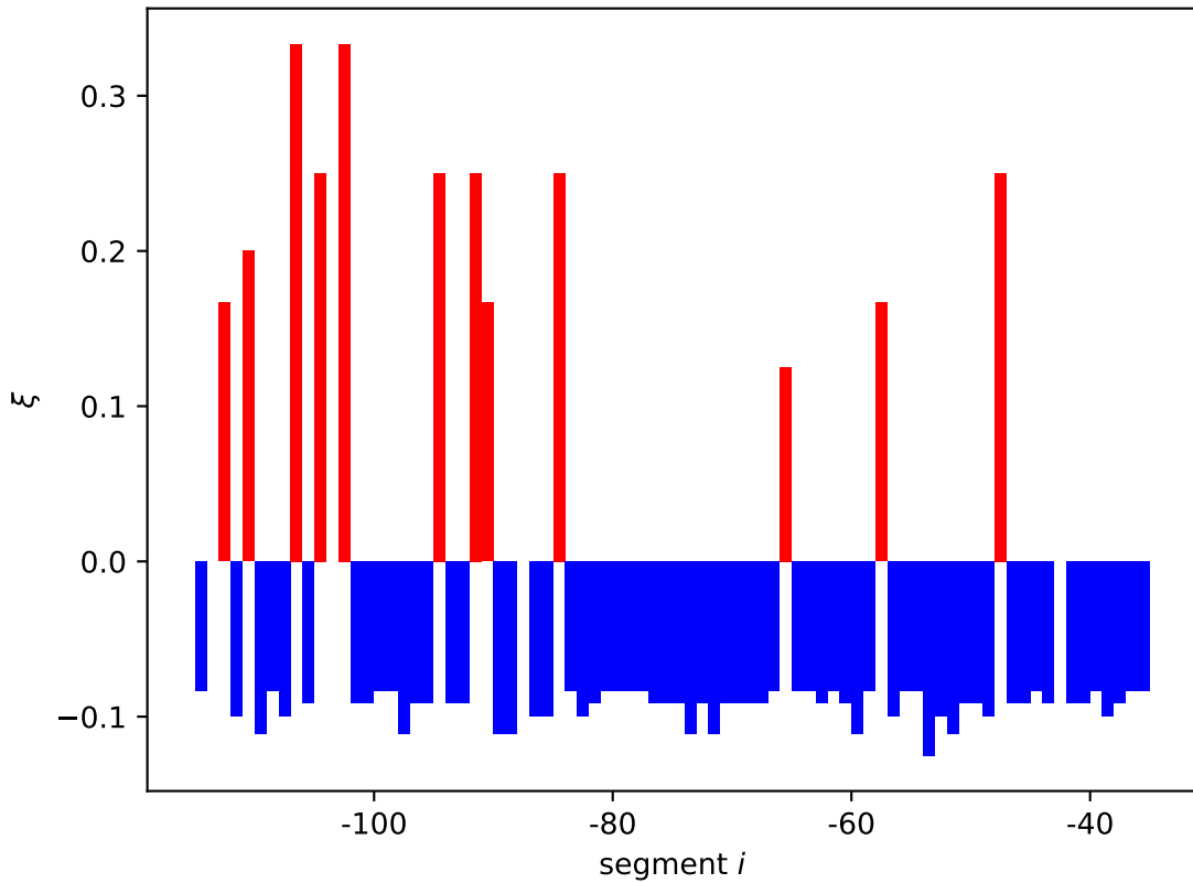
sdaB expression shift \xi_i[01, 10]
