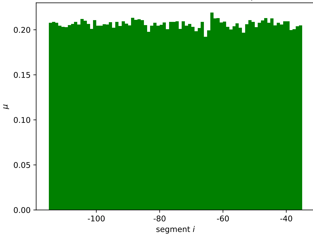
sdaB mean wildtype expression \mu_i^*
