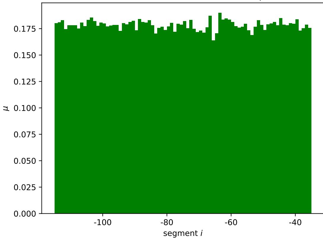
sdaB mean wildtype expression \mu_i^*
