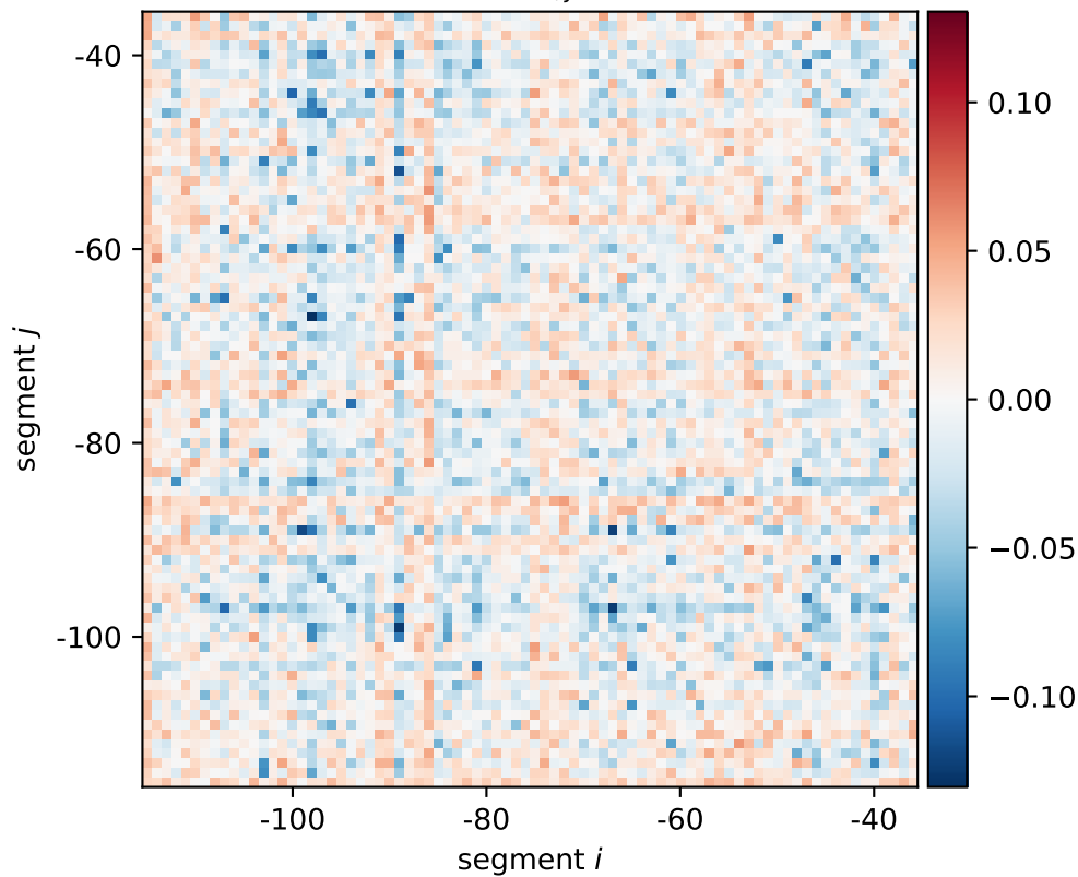
sdiA expression shift \xi_{i,j}[0101, 0110, 1010]
