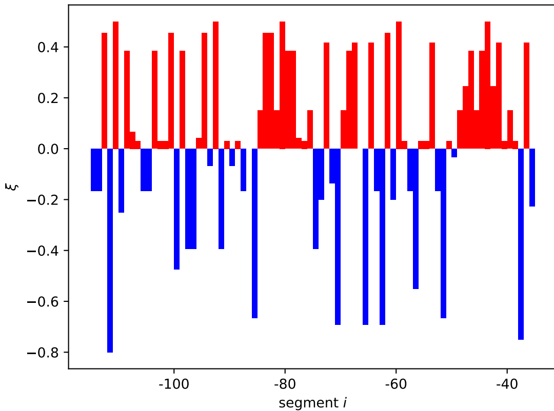
sdiA expression shift \xi_i[01, 10]
