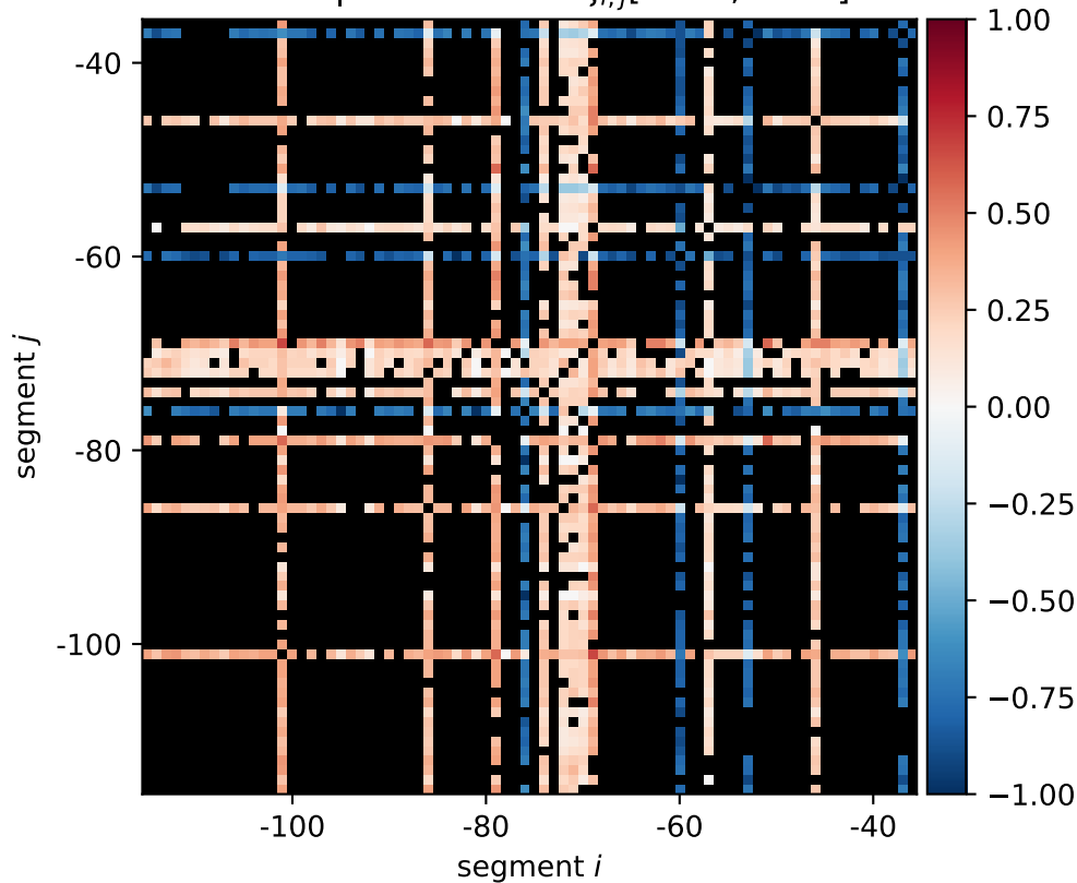
sdiA expression shift \xi_{i,j}[0011, 1100]
