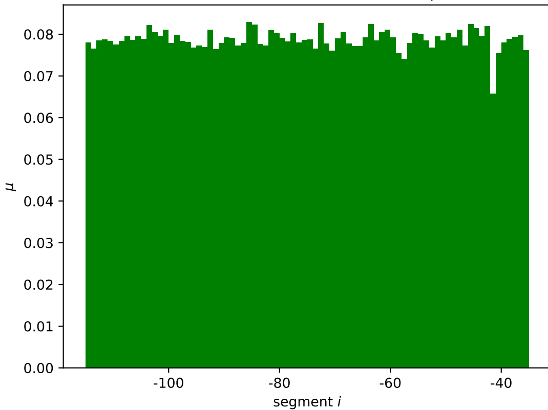
tar mean wildtype expression \mu_i^*
