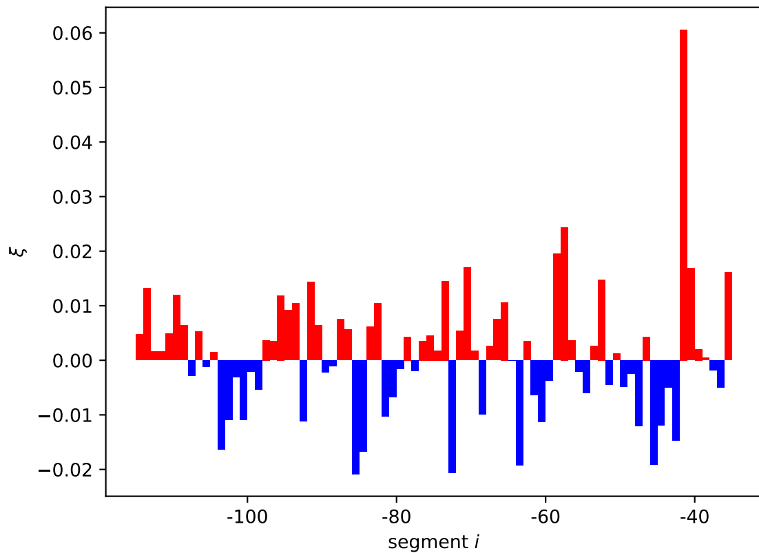
tar expression shift \xi_i[01, 10]
