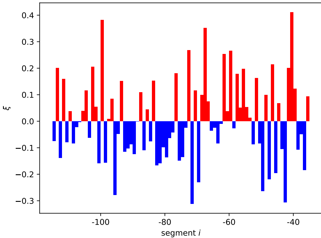
tar expression shift \xi_i[11]
