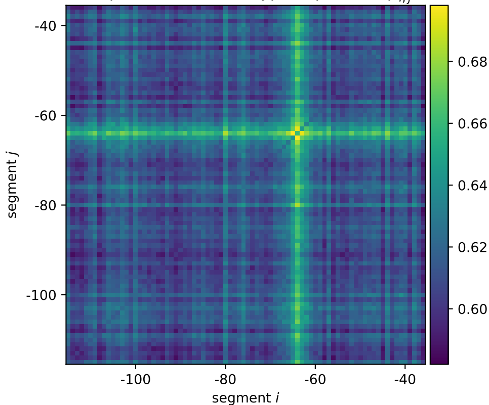
tff-rpsB-tsfc mean wildtype expression \mu_{i,j}^*
