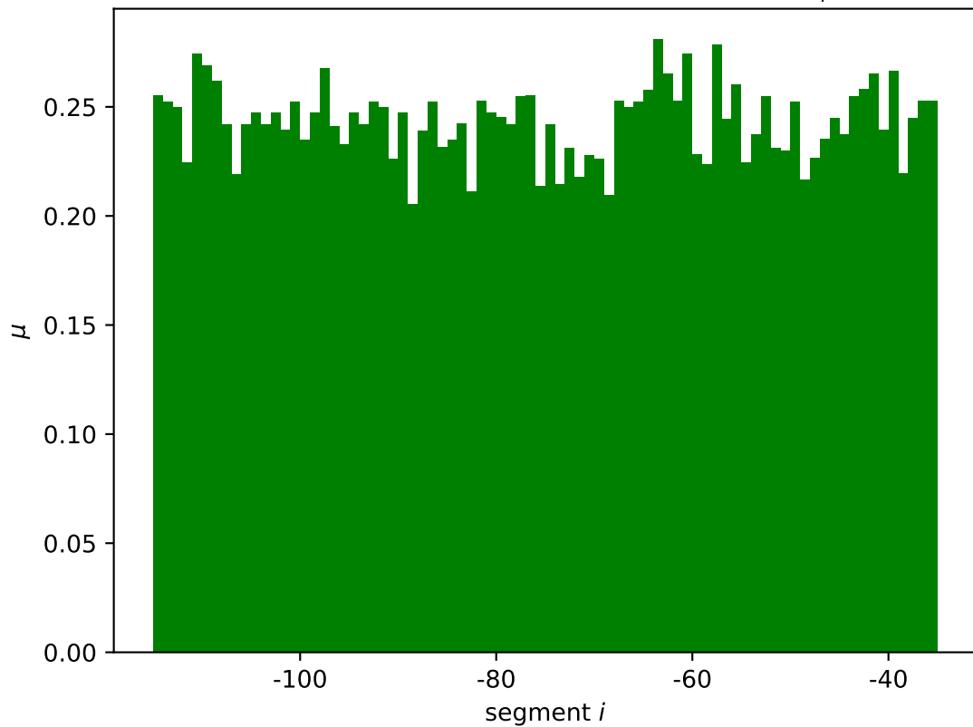
tff-rpsB-tsfc mean wildtype expression \mu_i^*
