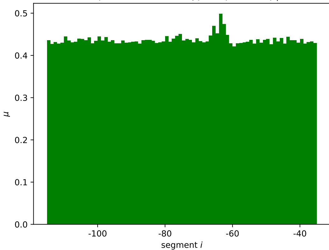
tff-rpsB-tsf mean wildtype expression \mu_i^*
