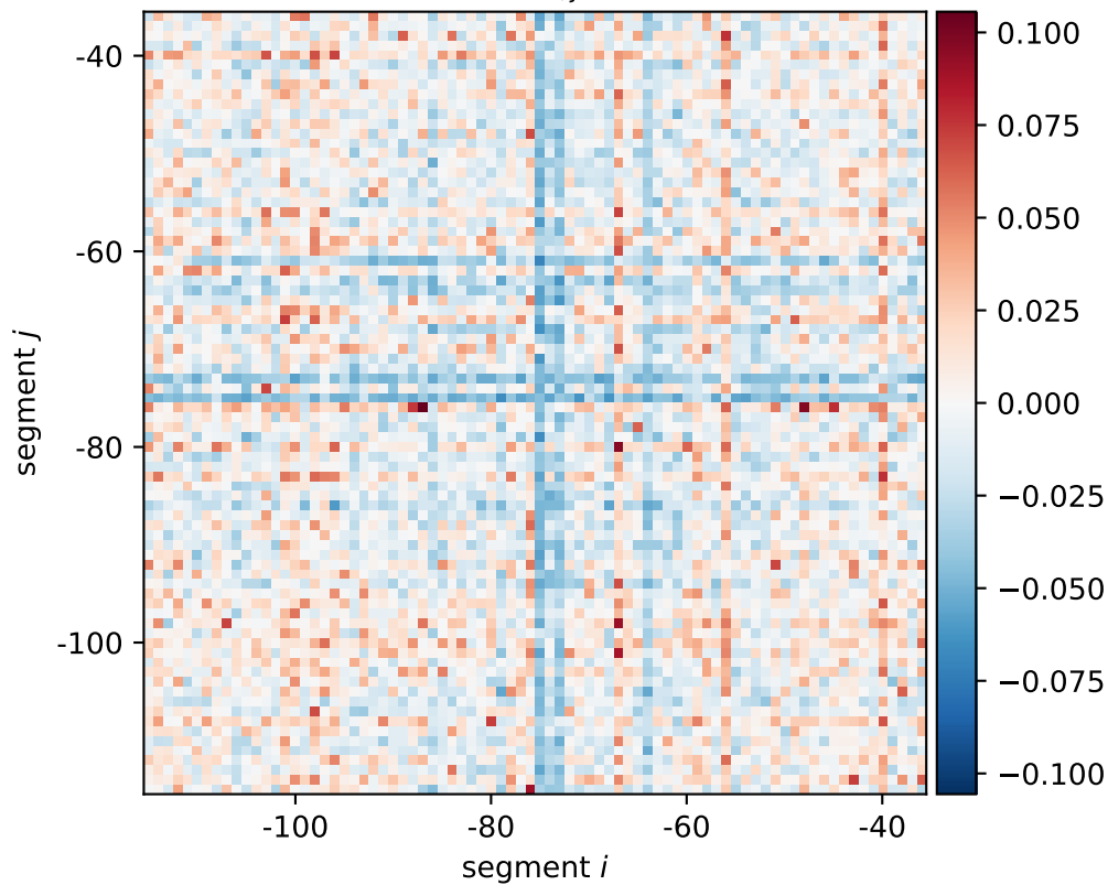
thiM expression shift \xi_{i,j}[0101, 0110, 1010]
