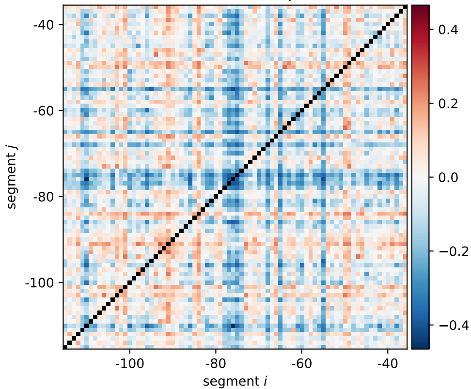
thrLABC expression shift \xi_{i,j}[0011, 1100]
