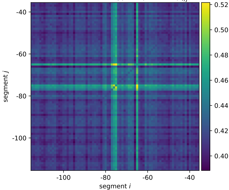
thrLABC mean wildtype expression \mu_{i,j}^*
