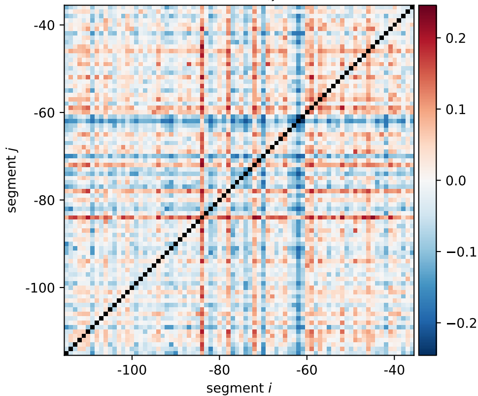
tig expression shift \xi_{i,j}[0011, 1100]
