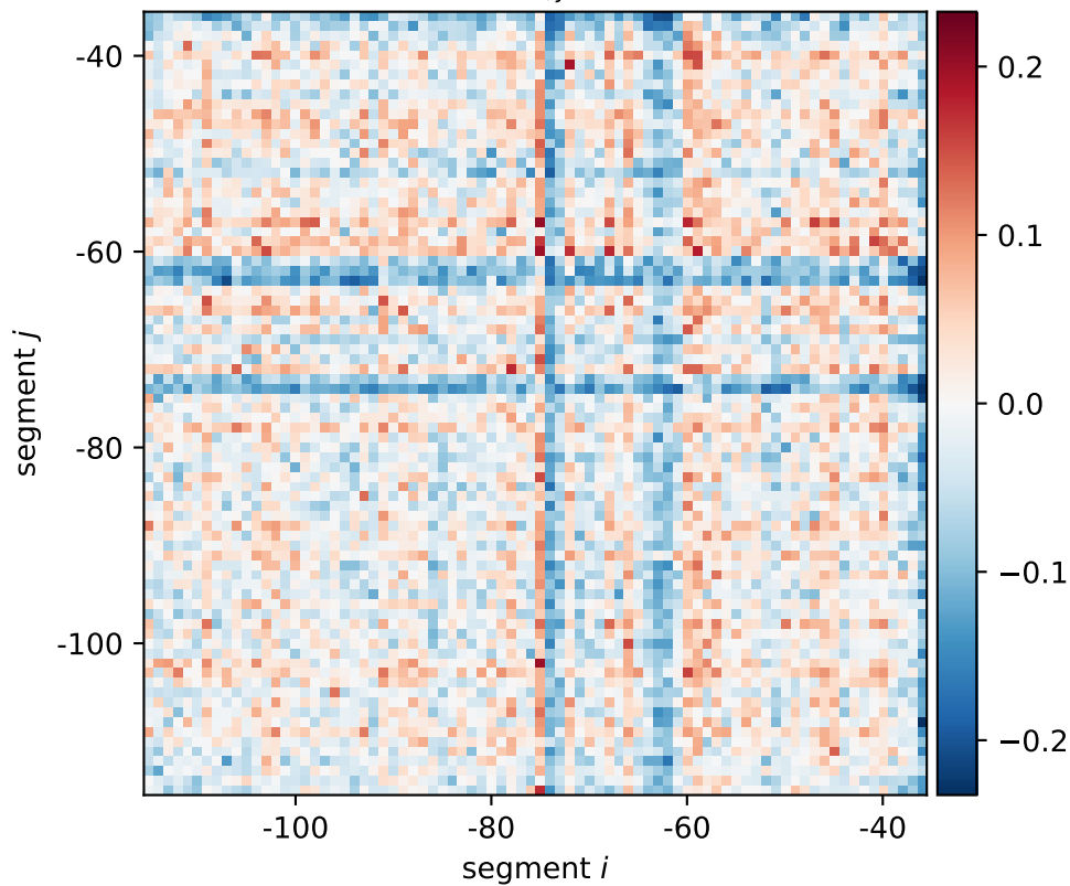
tig expression shift \xi_{i,j}[0101, 0110, 1010]
