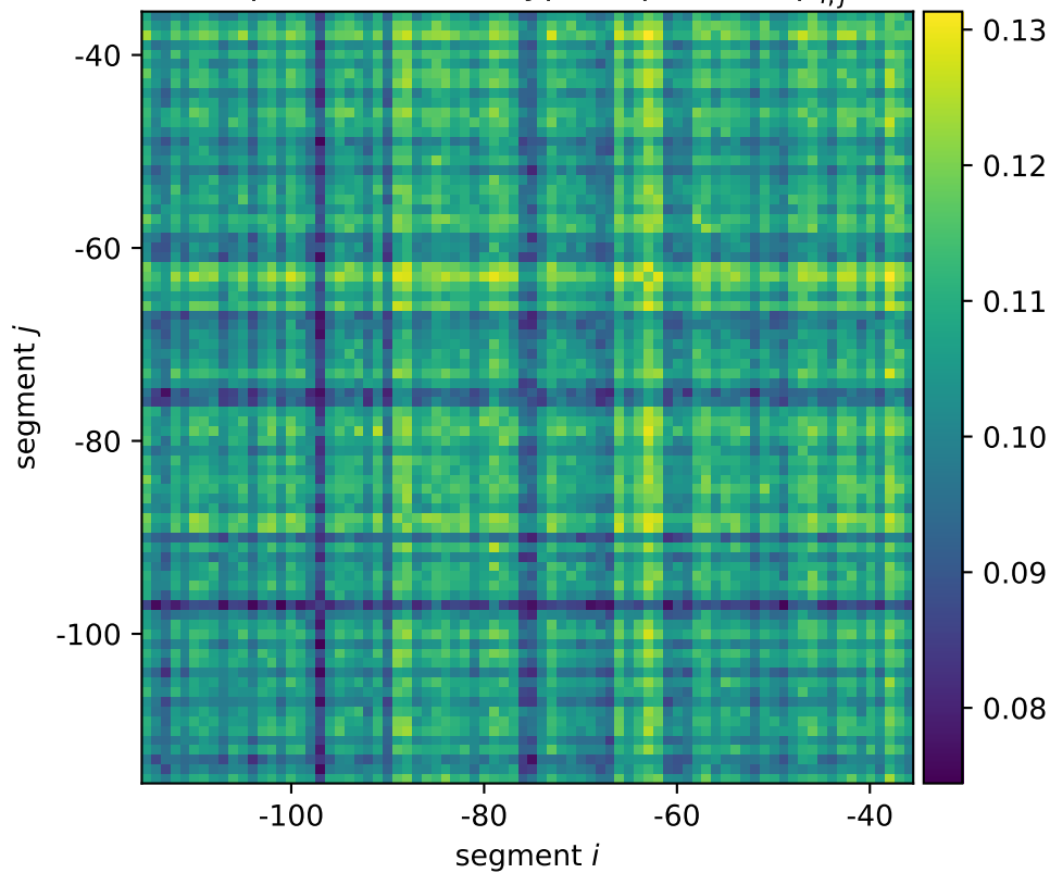
xapAB mean wildtype expression \mu_{i,j}^*
