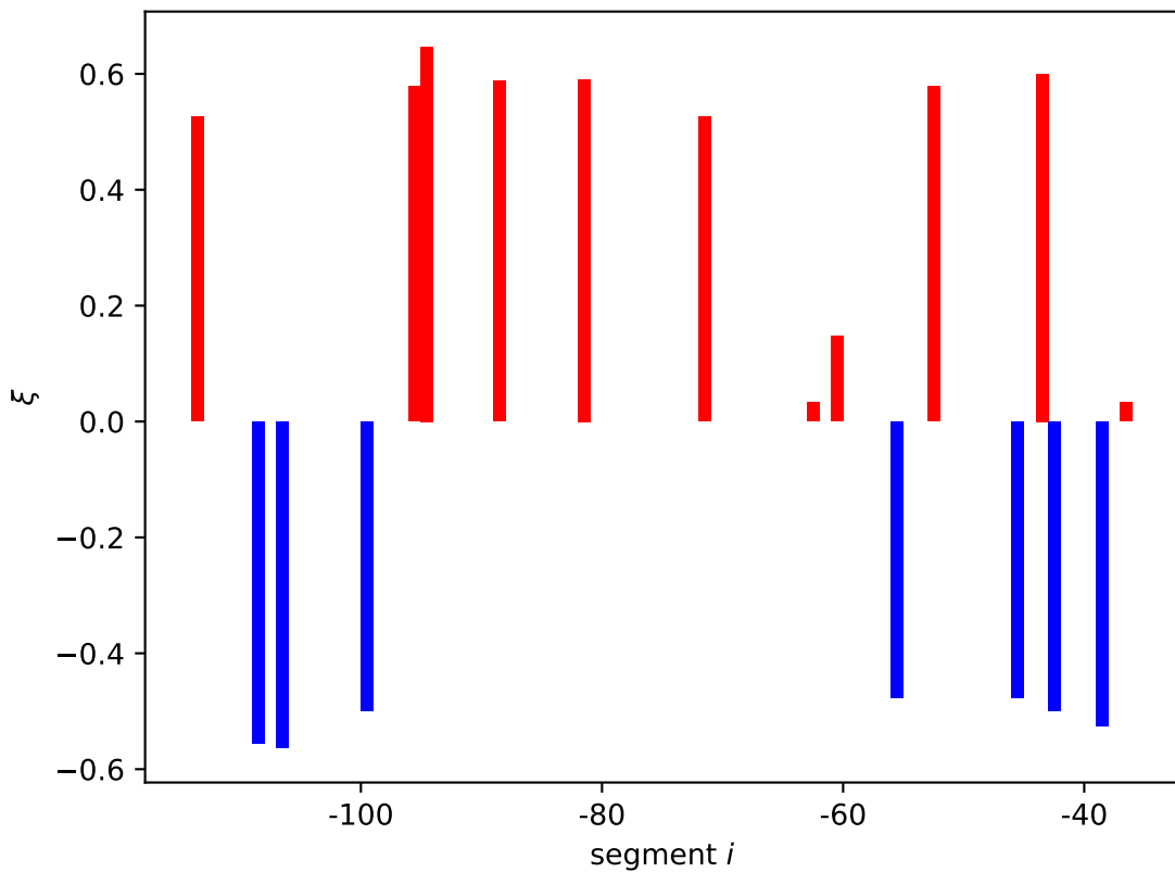
xylA expression shift \xi_i[11]
