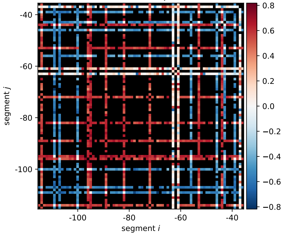
xylA expression shift \xi_{i,j}[0011, 1100]
