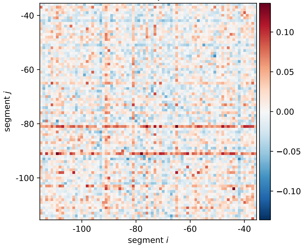
xylA expression shift \xi_{i,j}[0101, 0110, 1010]
