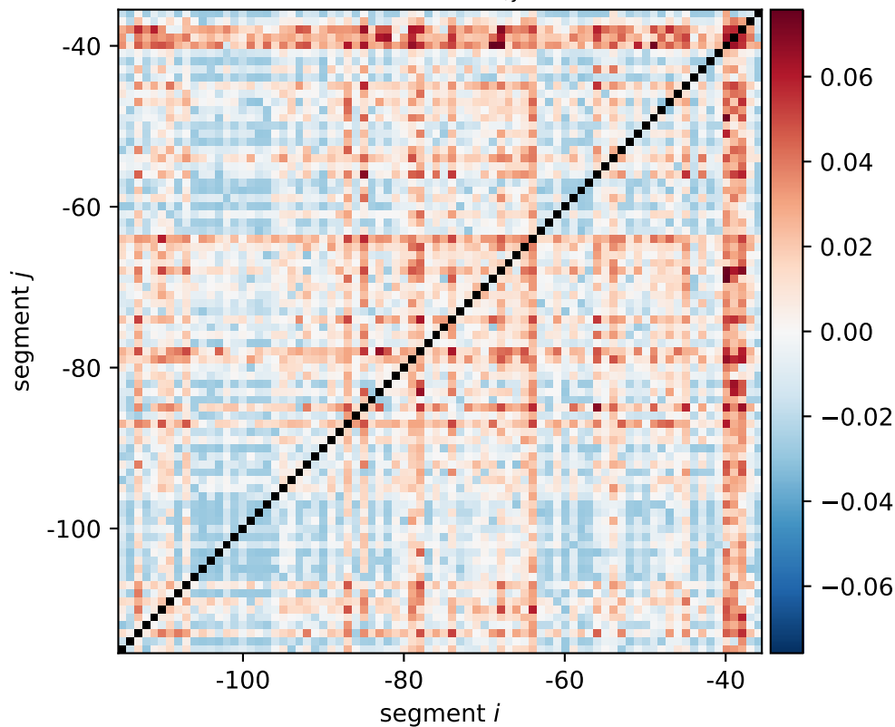
xyIF expression shift \xi_{i,j}[0011, 1100]
