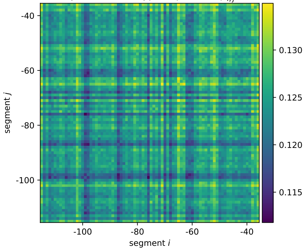
xylF mean wildtype expression \mu_{i,j}^*
