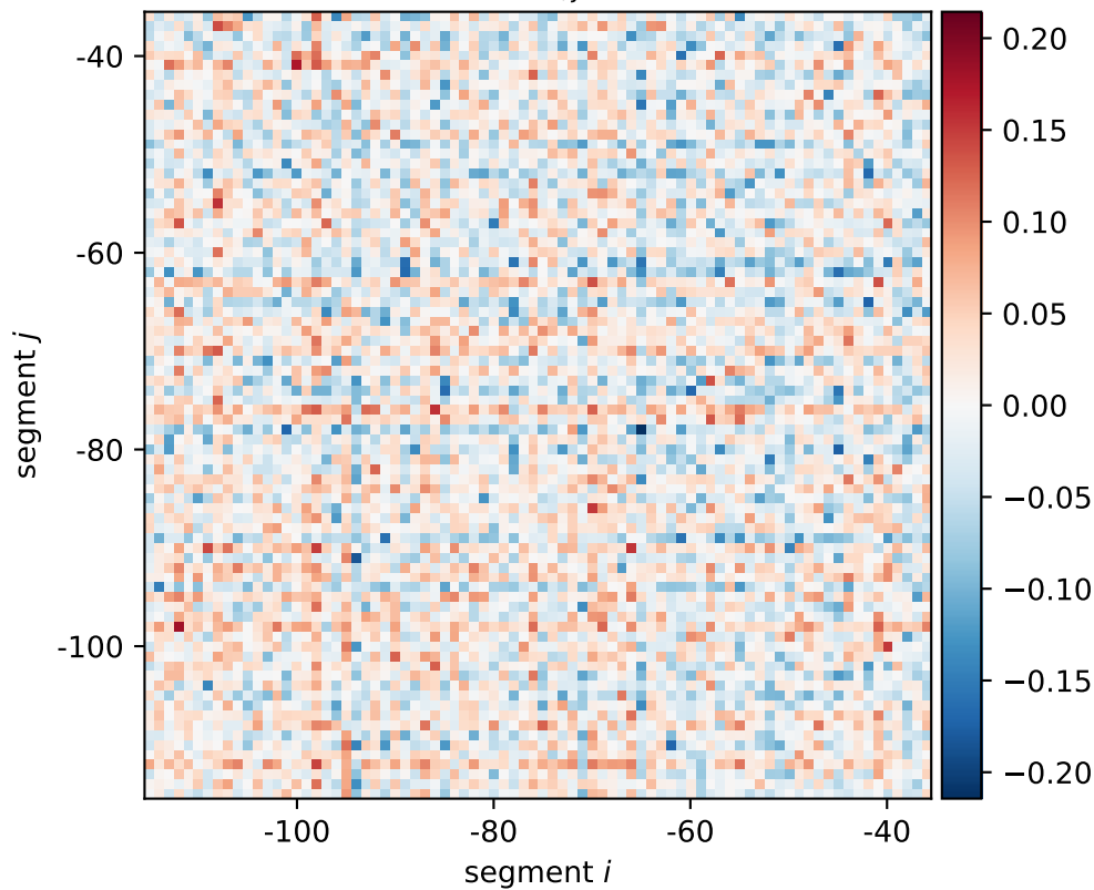
xyLF expression shift \xi_{i,j}[\text{0101}, \text{0110}, \text{1010}]
