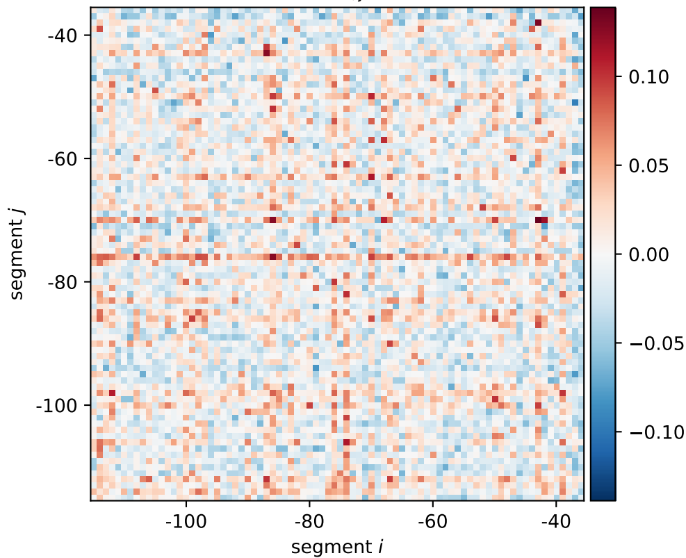
xyIF expression shift \xi_{i,j}[0101, 0110, 1010]
