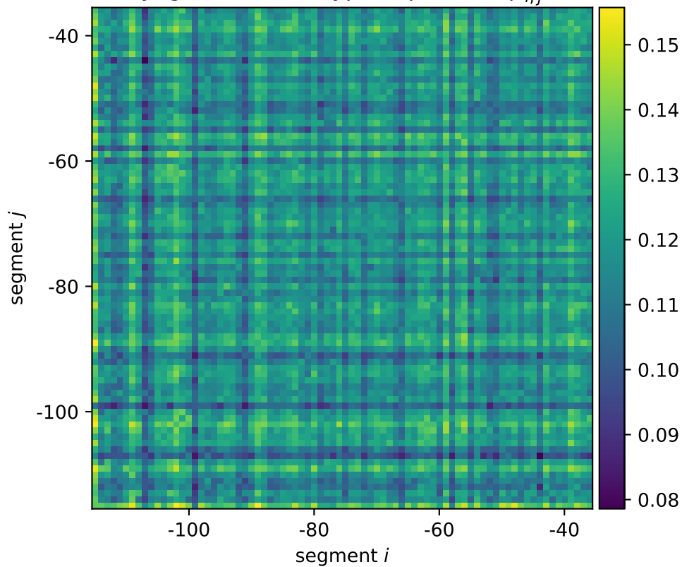
yagH mean wildtype expression \mu_{i,j}^*
