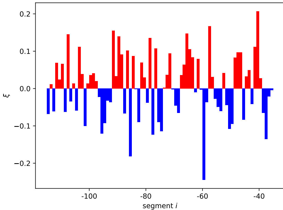
yagH expression shift \xi_i[01, 10]
