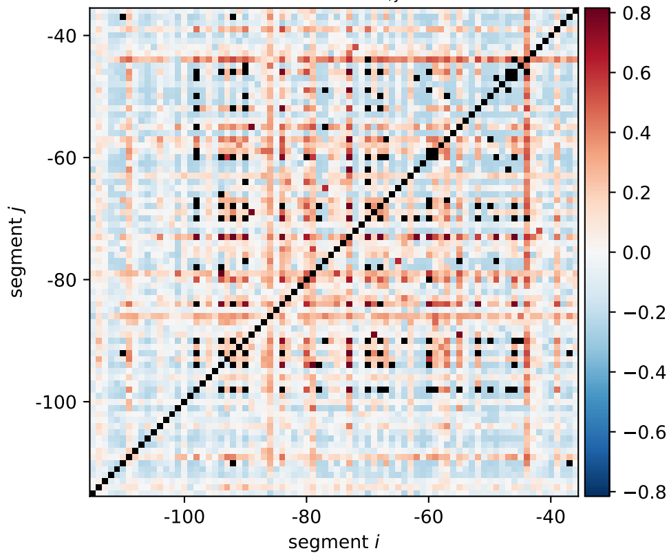
yagH expression shift \xi_{i,j}[0011, 1100]
