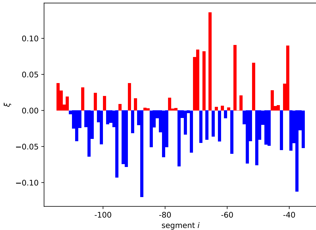
yagH expression shift \xi_i[01, 10]
